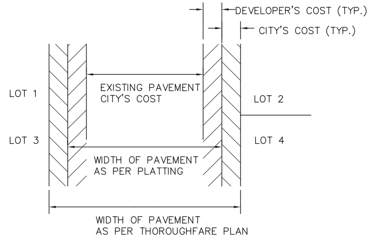
STREET IMPROVEMENTS FROM EXISTING STREET WIDTH TO THOROUGHFARE PLAN WIDTH
