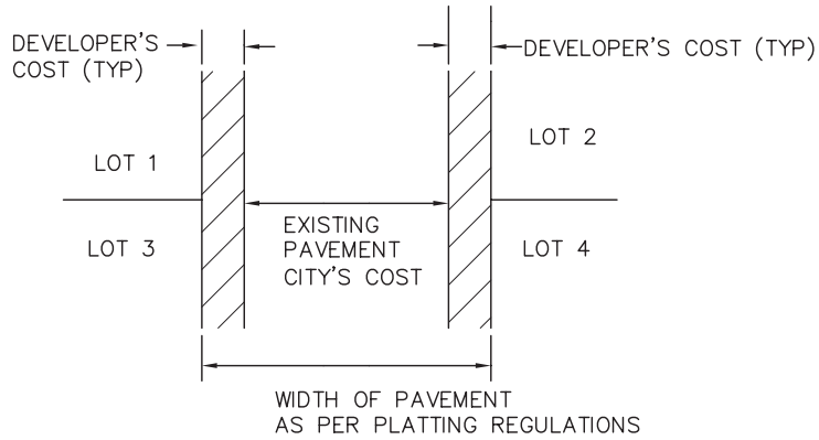
STREET IMPROVEMENTS FROM EXISTING STREET WIDTH TO PLATTING REGULATION WIDTH
